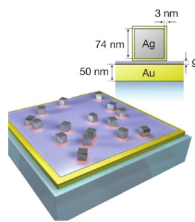
Figure 1: Gap-plasmon resonators constituted of silver nanocubes spread on a spacer deposited on a gold metallic surface [3]. Such structures are very efficient at concentrating and absorbing the incident light.
